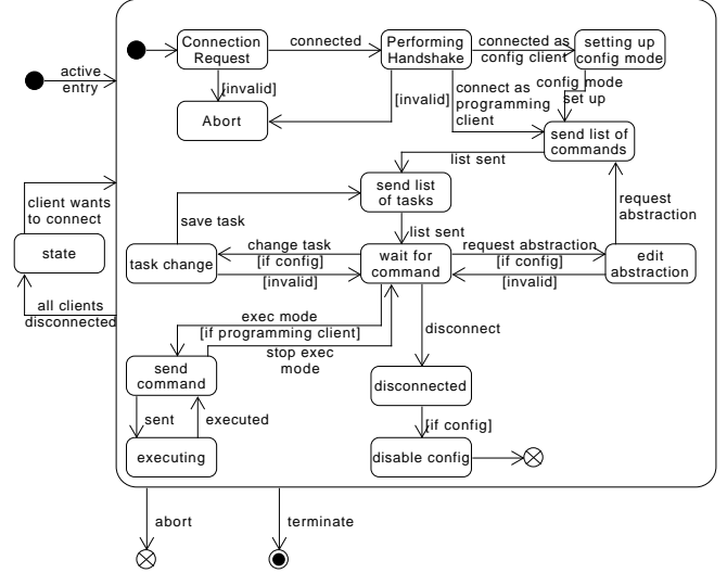
Fig. 2. A state transition diagram of the MiRACLE protocol
