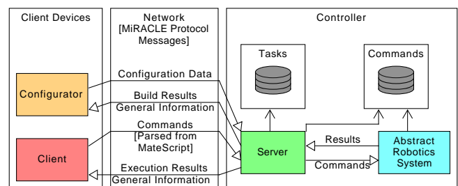
Fig. 1. The data flow between the sub-systems of MissionEDU
