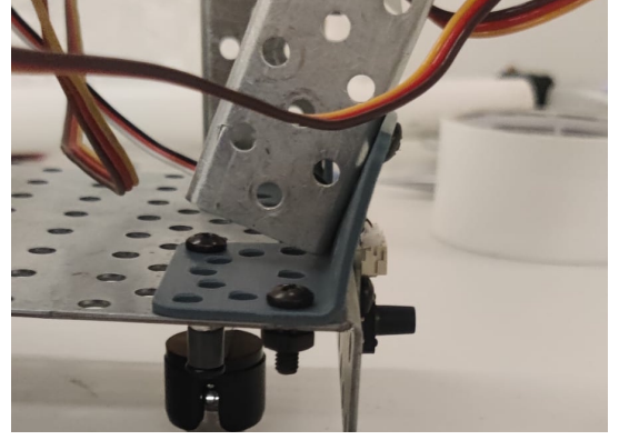
Fig. 6. Plastic Angle Bracket: Deflected Angle Bracket at Maximum Arm Extend ( \pm 0.5^\circ )
